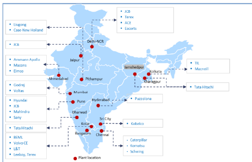
Figure 28 – Region-wise clusters
